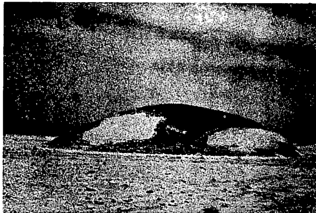
Fig. 14—Damage to responding concrete dome at 35-psi overpressure region, showing side of dome facing GZ.
